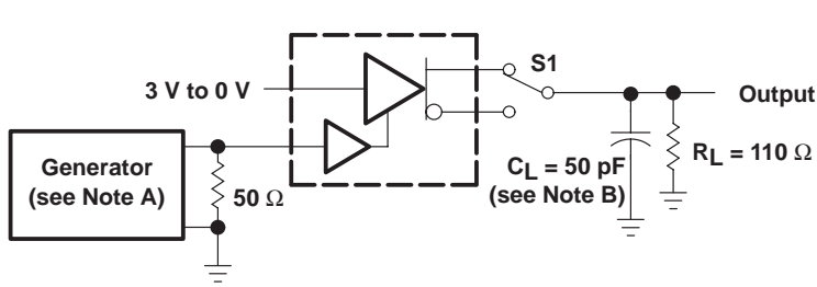
TEST CIRCUIT
